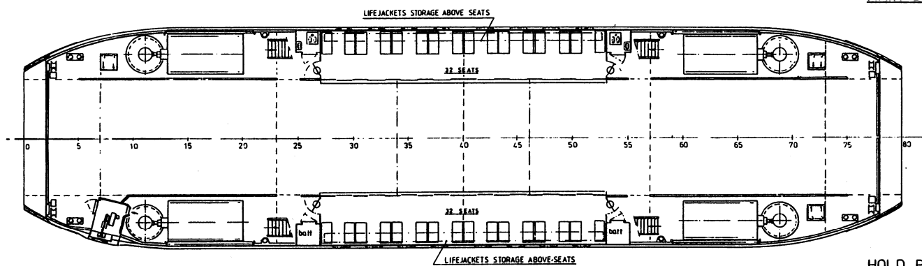
HOLD PLAN
