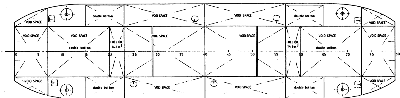
HOLD PLAN
