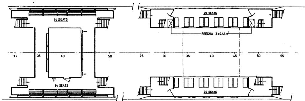
PASSENGER DECKS
